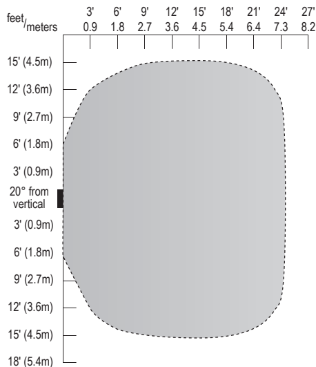
Figure 1. FS-505 coverage.
