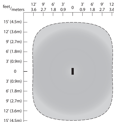
Figure 2. FS-505C coverage.
