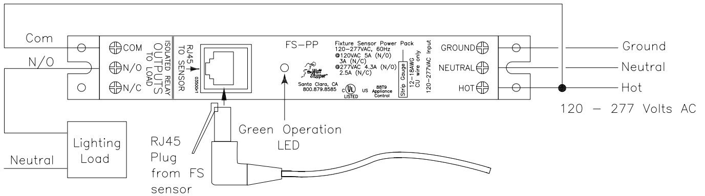
FS-PP Fixture Sensor Power Pack using N/O Relay for ON/OFF of Typical Load
