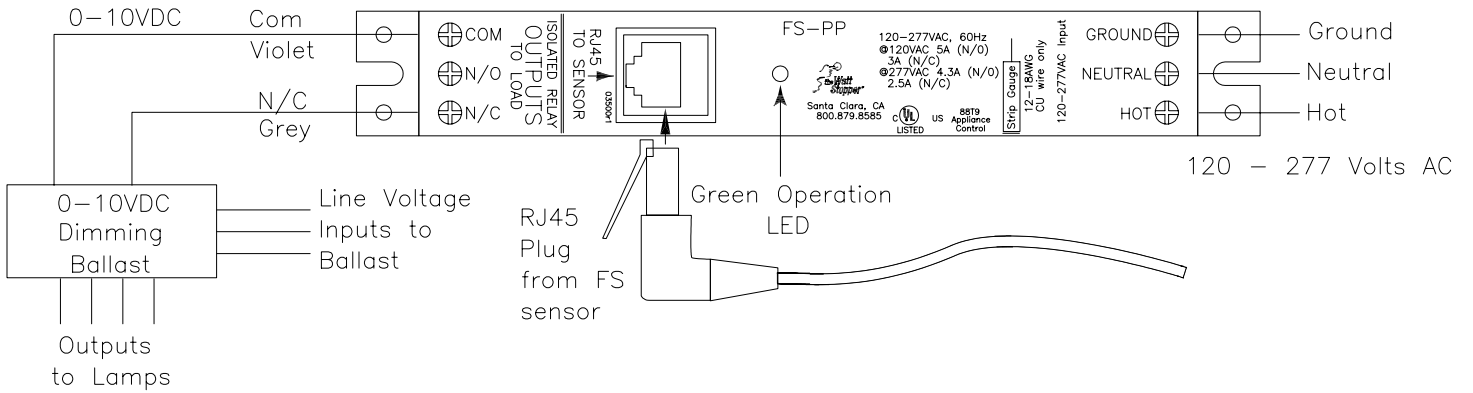
FS-PP Fixture Sensor Power Pack using N/C Relay for Hi/Lo control with (0-10vdc Dimming Ballast)
