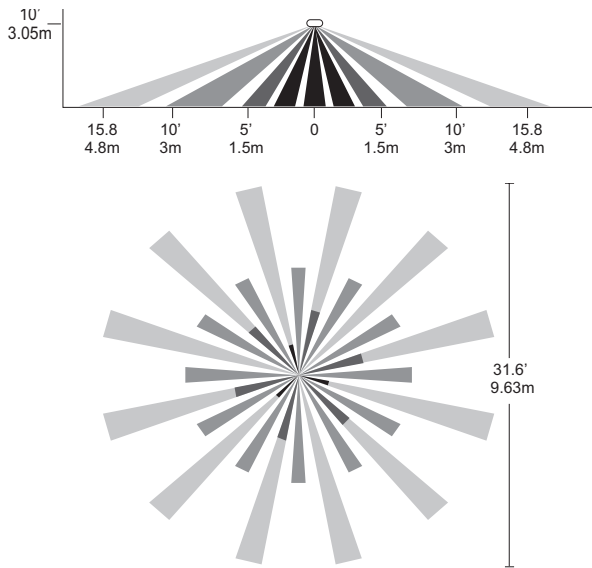
LMPC-600, wide angle/extended range lens
