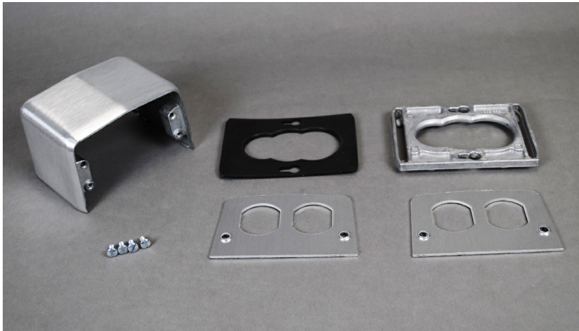
Four-piece power service fitting. Duplex opening both sides. Receptacles not included.
