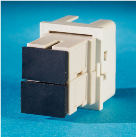
TracJack Module, 2-SC Simplex, Singlemode Blue Adapter, 180 degree exit, fog white
