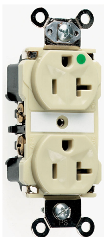
Extra Heavy-Duty Hospital Grade Duplex Receptacle Back and Side-Wire 20A 250V
