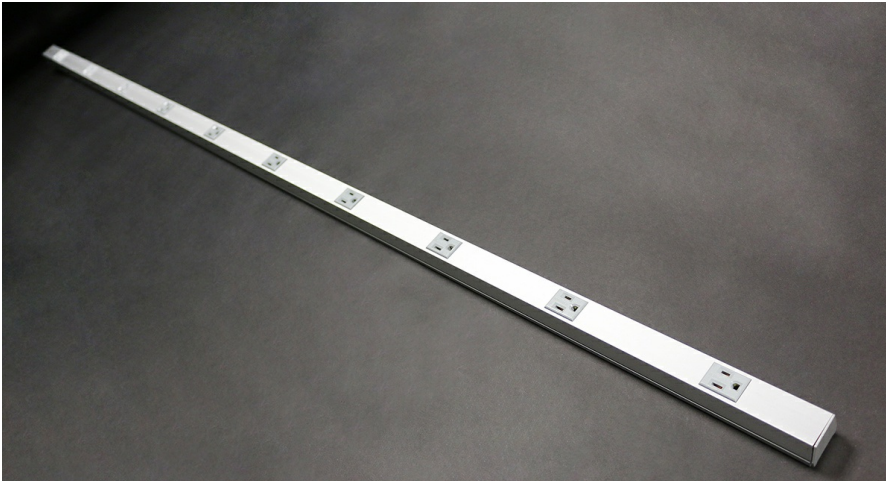
6' Aluminum Plugmold Multioutlet System comprised of twelve 6 inches apart, GBA
