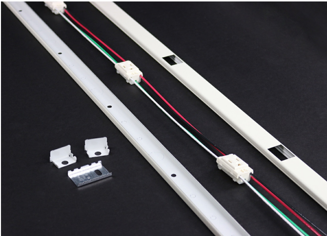
6' Plugmold Multioutlet System with 8 single outlets 12 inches apart, GBA
