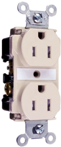
Tamper-Resistant Spec Grade Receptacles, Back and Side-Wire, 15A, 125A
