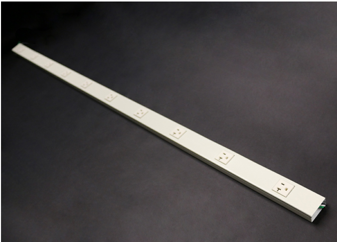
3' Steel Plugmold Multioutlet Strip with 6 single receptacles spaced 6"
