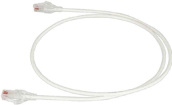
RDC 6 Modular Patch Cord, white, 7', reduced diameter, 28 AWG, cat6 channel four-pair UTP stranded PVC/CM.
