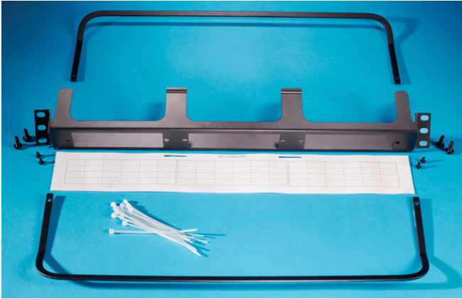
1U fiber patch panel for raised floor installation within floor box, for use with 45 degree angled mounting rails, holds 3 adapter panels
